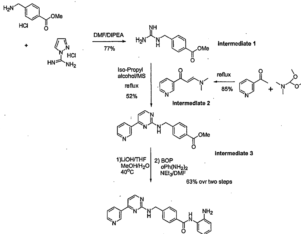
Scheme 66
